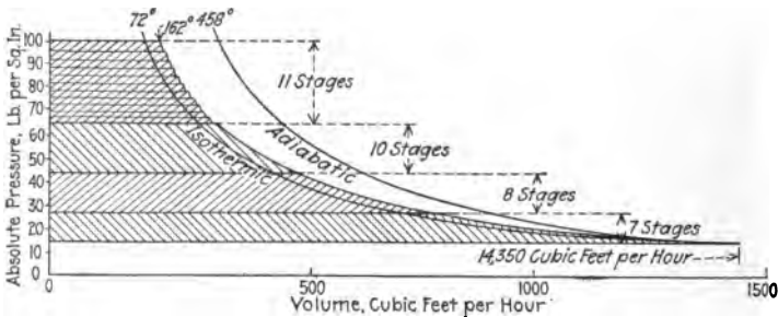
FIG. 90.—Diagram of tubo compression.
